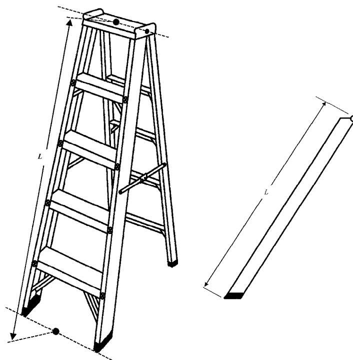
FIGURE W2 STEPLADDER WALKING TEST, Length L
