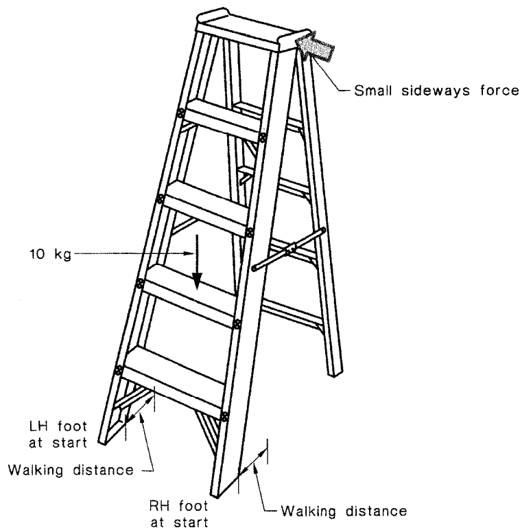
FIGURE W2 STEPLADDER WALKING TEST, Length L
